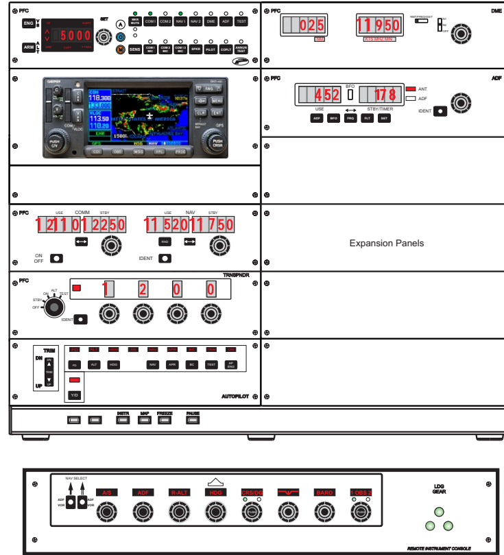
Optional configuration with Garmin GNS 430
