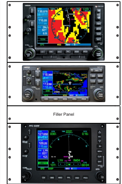
Optional Garmin GNS 530 GNS 430 PFC 530W
